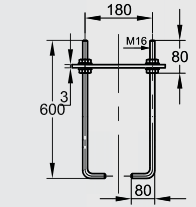
BASIC ANCHOR (Galvanized)
